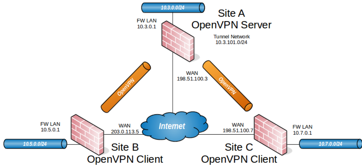
Fig. 68: OpenVPN Example Site-to-Site SSL/TLS Network
