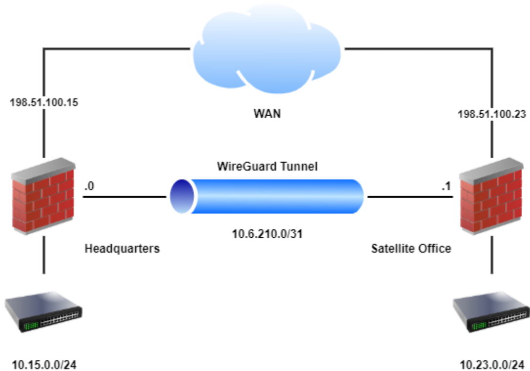
Fig. 84: WireGuard Example Site-to-Site Network
