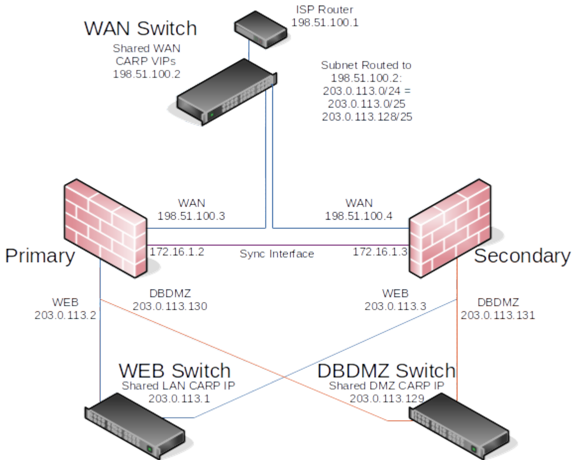
Fig. 11: Diagram of HA with Routed IPs
