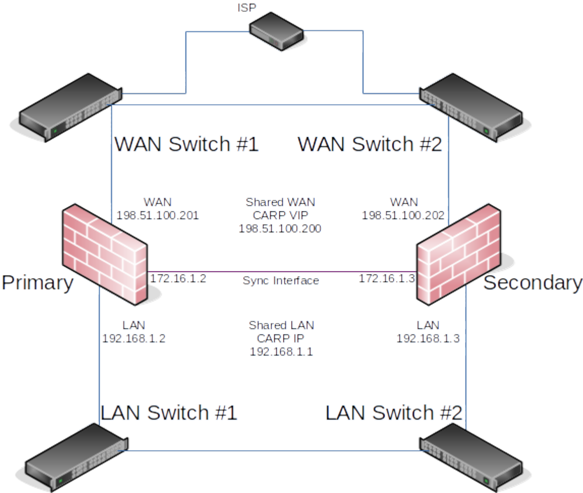
Fig. 3: Diagram of HA with Redundant Switches
