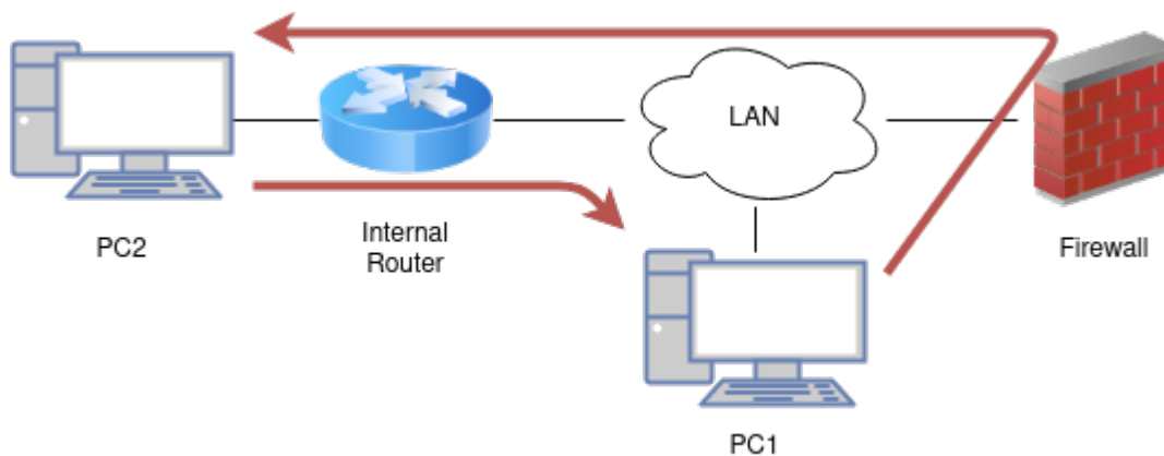
Fig. 3: Asymmetric Routing
