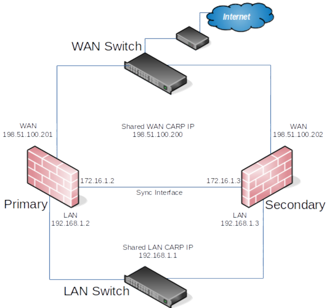
Fig. 6: Example HA Network Diagram
